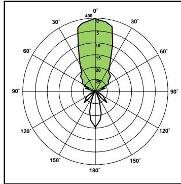
Polar Plot - DA-400 2.0 1/3 Octave @ 1 KHz
